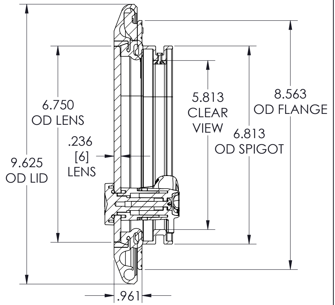
SECTION B-B
